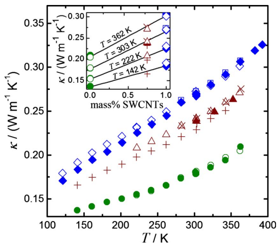
FIG. 1. (Color online) \kappa vs T for the PS matrix (2 samples: \bullet, \circ ) and 0.75 mass % SWCNT/PS (4 samples: \triangle, \times, +, \blacktriangle ) and 1 mass % SWCNT/PS (3 samples: \diamond, \square, \blacksquare ). The inset shows \kappa as a function of SWCNT content at selected temperatures.
