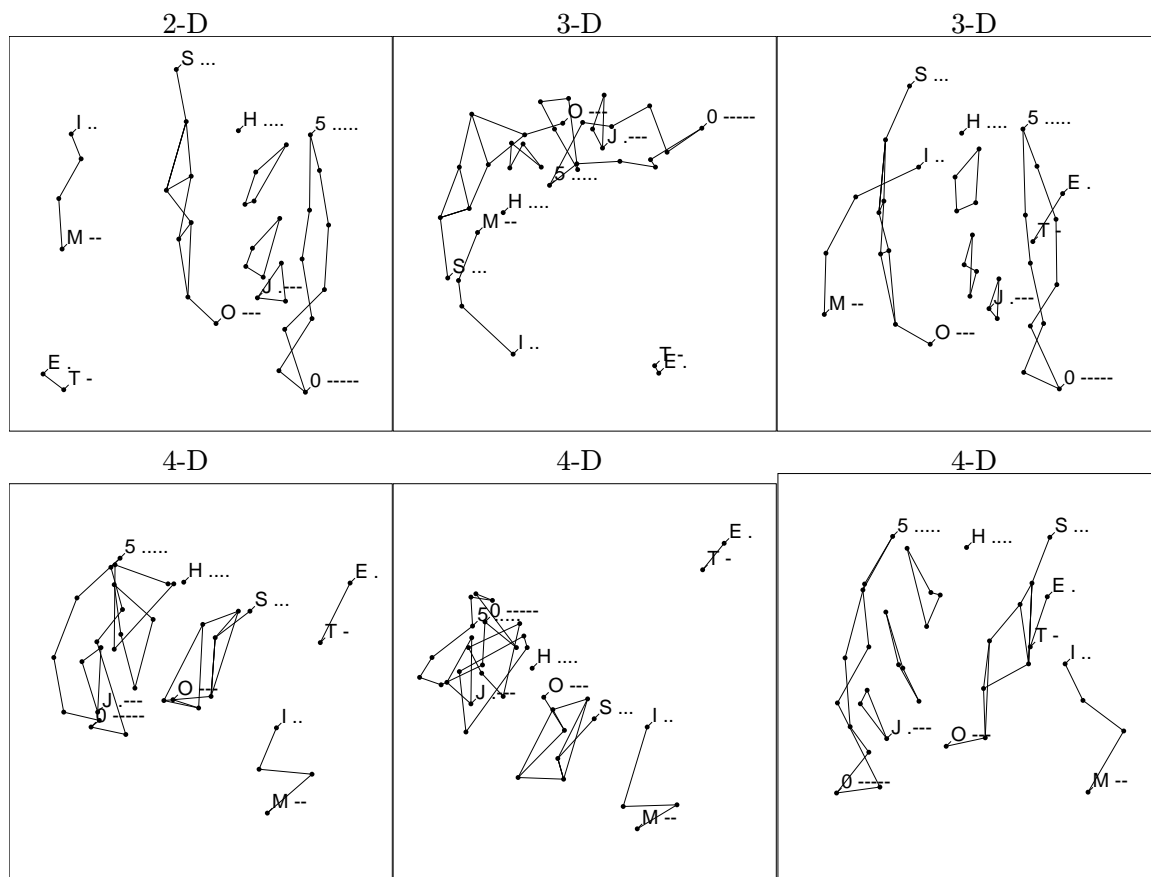
Figure 1: Views of Converged Nonmetric Scaling Solutions in 2-D, 3-D and 4-D. The stress values are 0.1874, 0.1254, and 0.0974, respectively. The second and the third frame show two projections of a 3-D configuration, and the frames in the bottom row show three projections of a 4-D configuration. The 3-D projections were obtained with 3-D rotations, the 4-D projections with so-called grand tours and manual tours.
