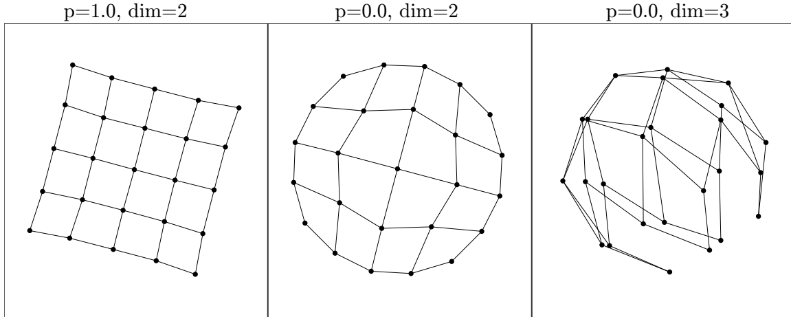
Figure 8: An Example of the Effects of Complete Indifferentionation on Metric MDS. The raw dissimilarities describe a 5 \times 5 grid as reflected in the 2-D configuration on the left. When subjected to the power zero, the dissimilarities become constants. The result are the 2-D configuration in the center and the 3-D configuration on the right.
