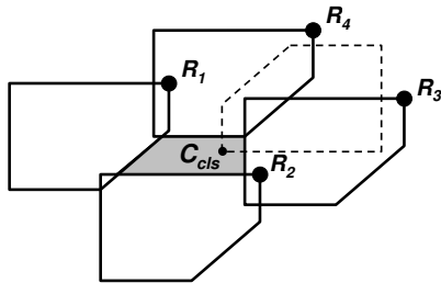
Fig. 3. Object closure: The interior (shaded gray) represents the closure configuration space , C_{cls} , for a team of 4 robots. The dashed polygon represents the object. Notice that the origin of the object's reference frame is inside C_{cls} , a compact set, indicating a condition of object closure.
