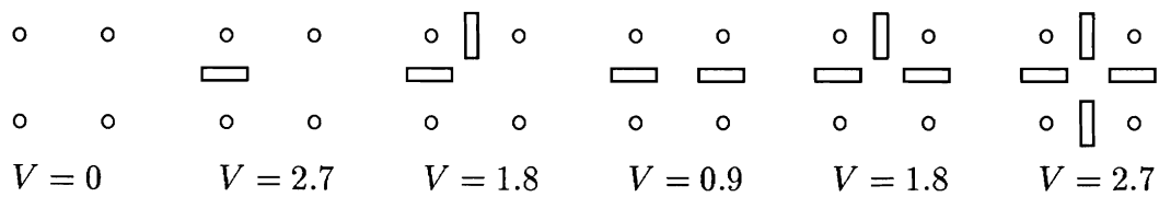
Figure 17: Original image: Hand-drawn. Potentials over the line process cliques.
