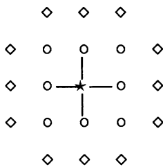
Figure 9: Posterior neighborhood.
