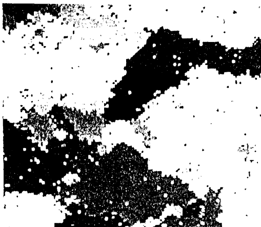
restoration: K = 25
