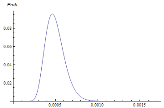
Likelihood function: P(u=271|a) for N=290
