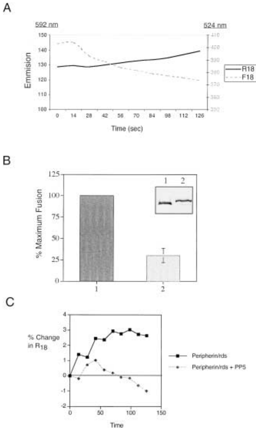
FIG. 6. Resonance energy transfer from F_{18} to R_{18} . (A) Presented above is a representative scan of the increase in R_{18} fluorescence emission at 592 nm (solid line) and the concomitant decrease in F_{18} fluorescence emission at 524 nm (dashed line) when F_{18} -labelled COS cell membranes containing peripherin/rds fuse with R_{18} -labelled ROS plasma membrane. The excitation wavelength is 460 nm. (B) Maximal fusion between R_{18} -labelled ROS plasma membrane and F_{18} -labelled COS cell membranes containing peripherin/rds or F_{18} -labelled disk membranes. The RET assay was performed as described in the 'Materials and Methods' and maximal percent fusion was calculated. Western blot analysis was also performed to confirm peripherin/rds expression in both samples (shown in inset). Inset, lane 1 disk membrane peripherin/rds; Western blot probed with monoclonal antibody 2B6 and lane 2, FLAG-tagged peripherin/rds in COS cell membranes; Western blot probed with anti-FLAG antibody. (C) The percent change in R_{18} fluorescence over time (in sec) upon energy transfer when R_{18} -labelled ROS plasma membranes are mixed with F_{18} -labelled COS cell membranes, in the presence [—◆—] and absence [—■—] of PP-5.
