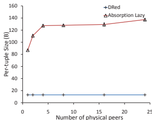
(a) Per-tuple Prov. Overhead (B)
