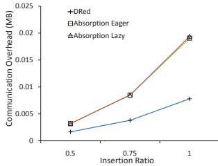
(b) Comm. Overhead (MB)
