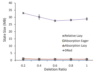
(c) State within operators (MB)
