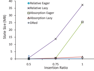
(c) State within operators (MB)
