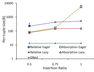
(a) Per-tuple Prov. Overhead (B)
