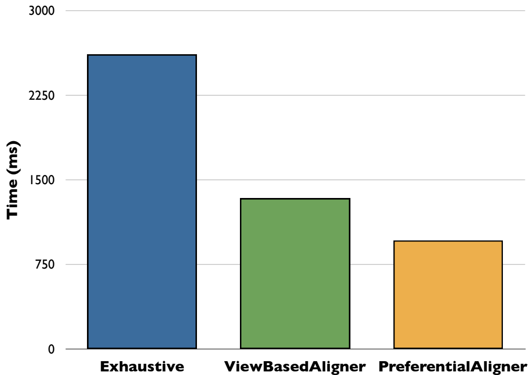
Figure 6.6: Running times (averaged over intro of 40 sources) when aligning a new source to a set of existing sources (COMA++ as base matcher). VIEWBASEDALIGNER and PREFERENTIALALIGNER significantly reduce running times vs. EXHAUSTIVE.
