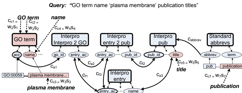
Figure 6.3: Query graph, given a series of keyword search terms. In general, each keyword may match a node with a similarity score s_{ci} , for which a weight coefficient w_{ci} is to be assigned by the system.
