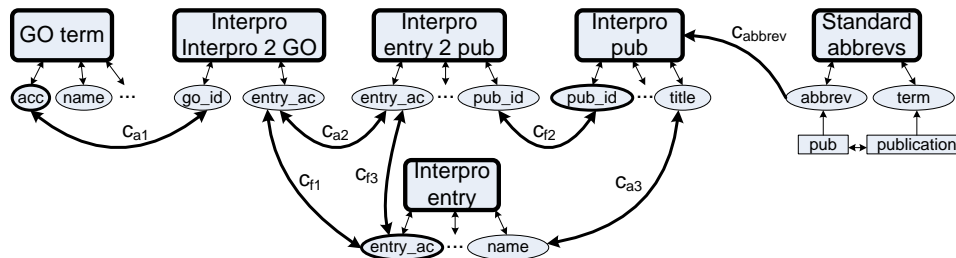
Figure 6.2: Search graph with weighted associations, indicated by bidirectional edges with cost terms c_i . Note the association between the table pub , the abbreviation pub , and the term publication , specified in the abbrevs table.
