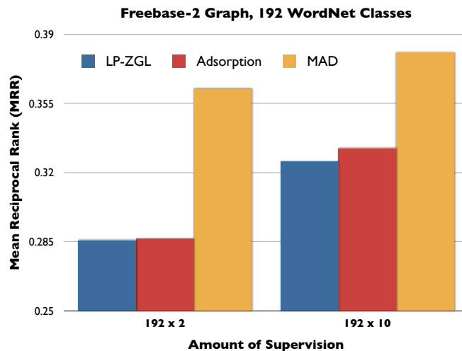
Figure 4.4: Comparison of graph transduction methods on a graph constructed from the Freebase dataset (see Section 4.6.2). All results are averaged over 10 random trials
