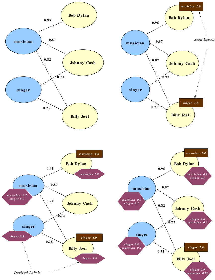
Figure 3.1: Section of a graph during various stages of the Adsortion label propagation algorithm. The initial graph without any labels on nodes is shown in the upper-left corner, while the final graph with labels estimated for all nodes using Adsortion is shown in lower-right corner. For better readability, instance nodes are shaded in yellow while class nodes are shaded in blue.
