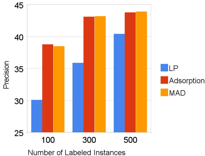
Figure 4.10: Precision for the Sentiment Analysis dataset with 3568 testing instances. All results are averages over 4 randomly generated transduction sets.
