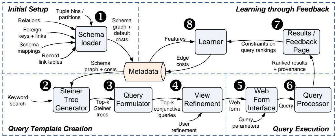
Figure 5.2: Architectural stages of the Q System.
