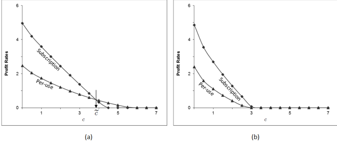
Figure 2. Profit rates of the two pricing schemes with respect to the capacity cost, c . The following parameter values are used: (a) w = 0.05 ; and (b) w = 0.5 . ( \Lambda = 1 and \bar{v} = 10 in both panels.)
