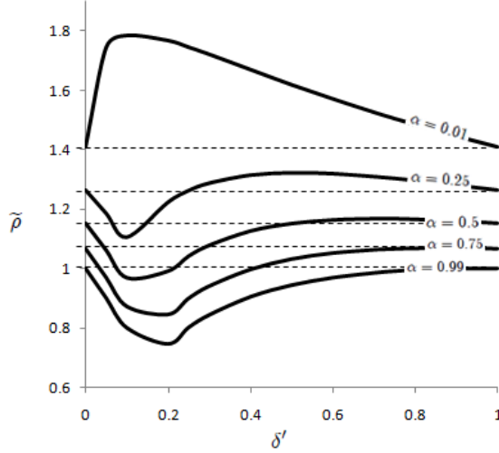
Figure 4. Potential utilization rates, \tilde{\rho}(\alpha, \delta') , that yield identical revenue with per-use and subscription pricing when consumers are heterogeneous.
