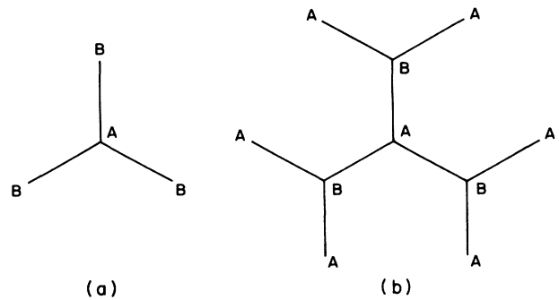
FIG. 7. Two-sublattice Cayley tree for \sigma=2 and with the origin on an A site, consisting of (a) one generation, (b) two generations.
