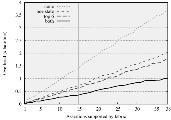
Figure 9: Hardware overhead with respect to the number of assertions supported by the configurable assertion fabric, evaluated at four optimization levels. The vertical line represents the number of Assert blocks required to implement the seven assertions needed to detect all of our attacks. 38 is the number of Assert blocks to implement all invariants.
