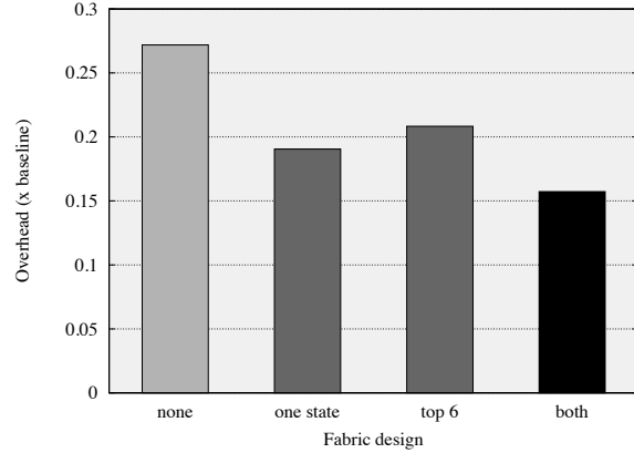
Figure 10: Timing delay overhead, averaged across all fabric sizes, with respect to the number of assertions supported by the configurable assertion fabric at four optimization levels.
