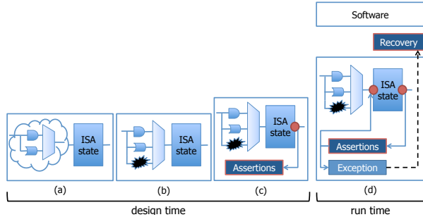
Figure 1: Processor design flow with MAGICCARPET: (a) Hardware description language implementation of the instruction set, with unintentional bugs. (b) Malicious designer adds intentional errors to the processor. (c) MAGICCARPET is added to the design as the last action [62], with taps directly on the outputs of ISA state storing elements. (d) MAGICCARPET dynamically verifies properties encoded into the fabric, triggering the recovery firmware in the event of a violation.
