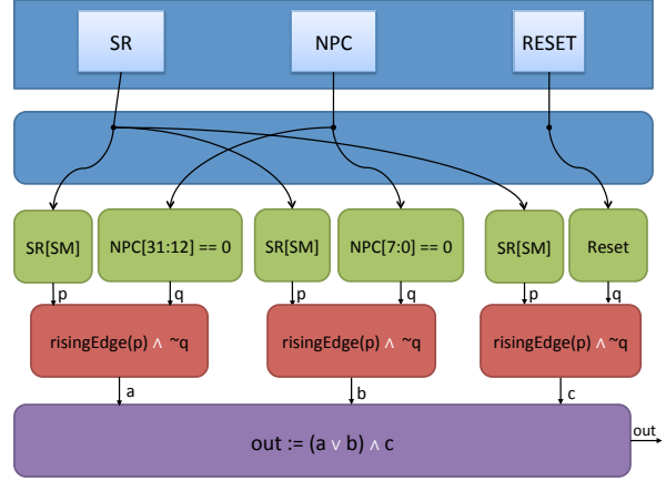
Figure 5: Fabric configured with a macro assertion that detects incorrect privilege escalations.
