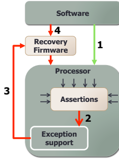
Figure 3: Detection and recovery in MAGICCARPET: 1) Software runs while assertions implemented in verified hardware check the processor’s state for specification violations; 2) A violation triggers an exception; 3) In-flight contaminated state is flushed and control passes to verified recovery firmware; 4) The ISA-level state is backed up, and firmware fetches, decodes, recodes, and executes a software simulation, then loads updated ISA-level state from the simulation into the processor and returns from the exception.
