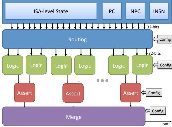
Figure 4: MAGICCARPET fabric: the Routing block sends ISA-level state elements to the Logic blocks; the Logic blocks condense multi-bit state and constant inputs down to a single bit output that is sent to the Assert block; the Assert block compares the previous value of its inputs to the current value, outputting the result as a one bit value to the Merge block; the Merge block combines the Assertion block results to form a higher-level result that indicates if the programmed invariants still hold; this result is tied to the processor’s exception generation logic.
