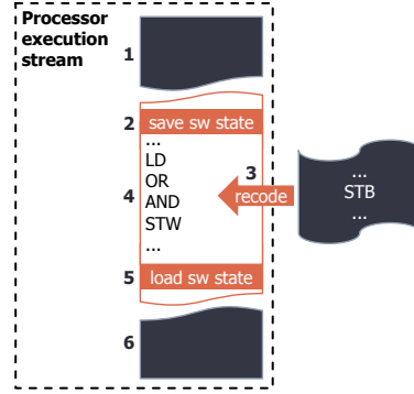
Figure 8: MAGICCARPET’s recovery mechanism: 1) Software executing normally on the processor 2) When the configurable assertion fabric detects a processor invariant violation, control passes to the recovery firmware which backs-up the software’s state and exception registers. 3) The recovery firmware fetches, decodes, recodes, and 4) executes several instructions from the software level. 5) Once past the error, the recovery firmware loads the processor with the software state in the simulator and passes control back to the software level. 6) Software resumes normal execution
