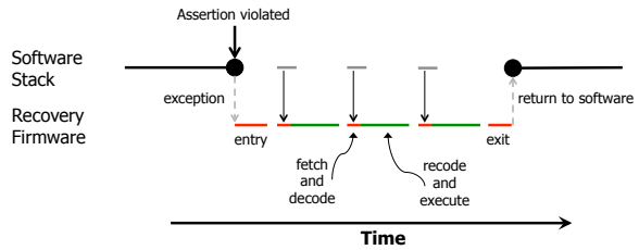
Figure 2: Recovery in MAGICCARPET: A property violation invokes the recovery firmware. Recovery is a repeated process of fetching an instruction from software, decoding it, and then executing the recoded instruction stream. The recovery firmware returns control back to software when it reroutes execution around the exploitable defect. The green/light portions of the recovery firmware’s execution are formally verified , while the red/dark portions are not. The fabric monitors the firmware’s execution.
