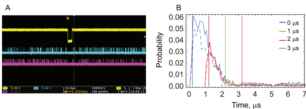
Figure 5.7: APD and gate pulse filter. (A) the APD pulses in APD x (cyan) and APD y (magenta) are AND-ed with the gate pulse (yellow) so that only photons that arrive after the short gate pulse are recorded. (B) Experiments similar to Fig. 5.6B using HVPS2 with 0 pF capacitance with a varying duration gate pulses (0-3 \mu s) to exclude photons that arrive within that interval immediately after the Pockels cell changes voltage. Subsequent experiments were performed with a 3 \mu s gate pulse.
