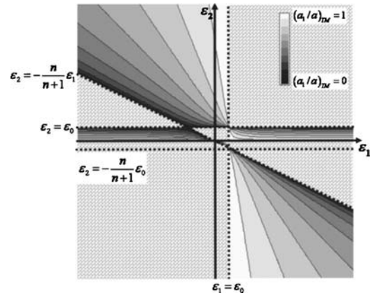
FIG. 3. Regions for which the transparency condition (14) for the TM-polarized scattered wave is fulfilled, with the corresponding values for a_1/a between zero and unity. Analogous to Fig. 2, the forbidden regions indicated with the brick symbols correspond to values of \varepsilon_1 and \varepsilon_2 for which the condition (14) for the TM case has no physical meaning.
