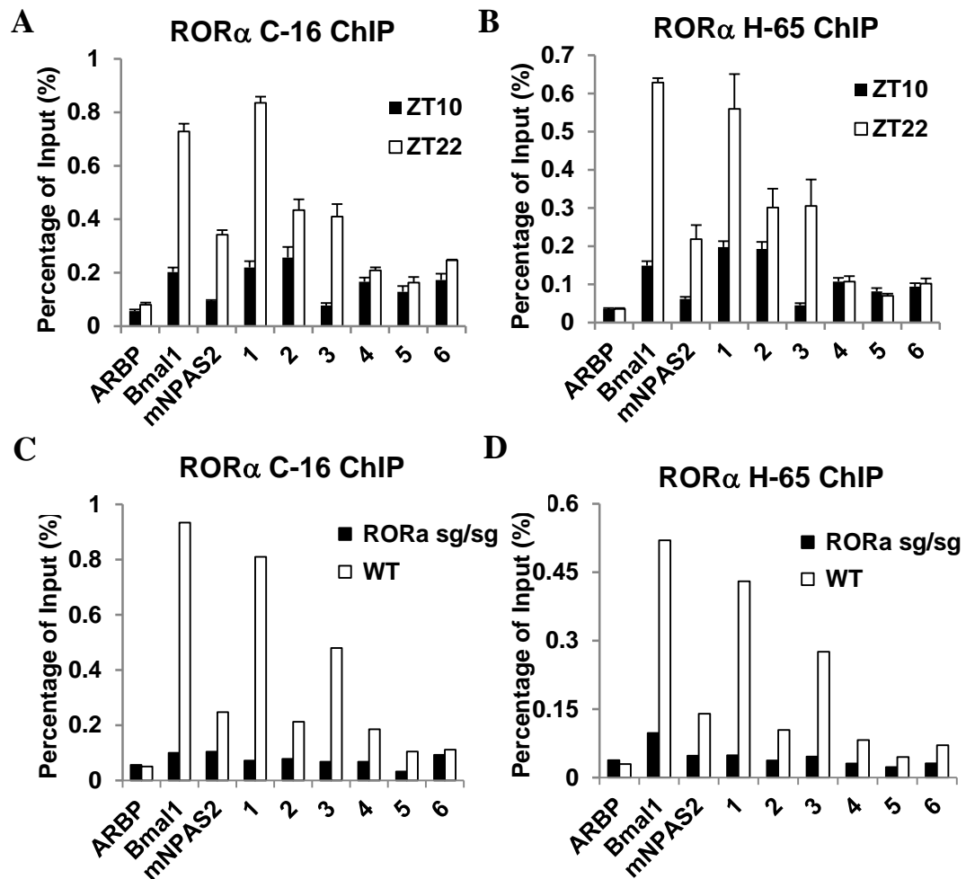
Figure 4.10 Validation of ROR \alpha Binding Sites.
