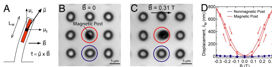
Fig. 2. Characterization of magnetic post actuation. (A) The magnetic torque, \tau , on a magnetic post of length L_w and dipole moment, \bar{\mu} . (B and C) Phase-contrast micrographs of a magnetic post deflected under no field and a 0.31-T field. (D) Plots of post displacement versus applied field with arrows indicating direction of driving magnetic field. Actuations caused negligible mechanical displacement in adjacent nonmagnetic post (blue curve).
