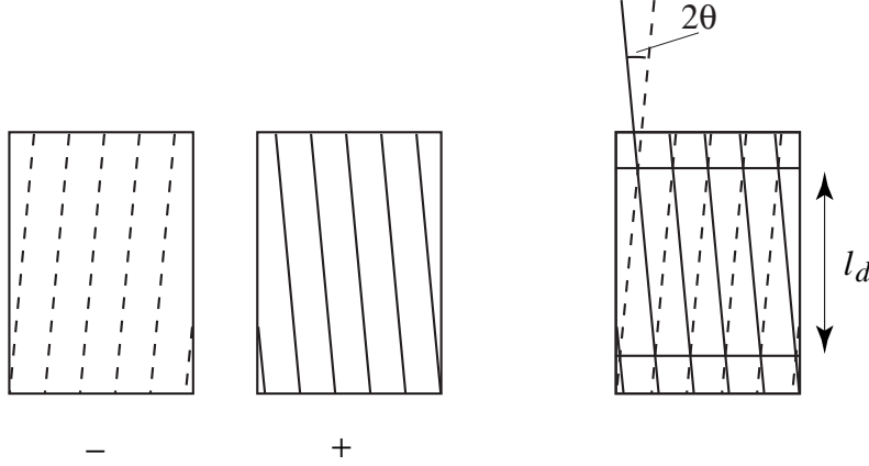
Figure 6: Creation of a twist grain boundary at the interface between two cells. All cells twist in the same direction. The columns in back (-) and in from (+) of a given interface twist in opposite directions. The interface is thus a twist grain boundary consisting of screw dislocations perpendicular to the z axis separated by a distance l_d = d/2 \sin \theta , where 2\theta is the change in angle of the columnar lattice across the boundary.
