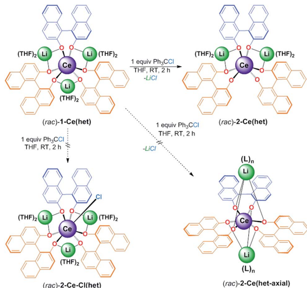
Scheme 4 Oxidation of 1-Ce(het) with Ph_3CCl to produce salt-elimination product, 2-Ce(het). Other previously observed oxidation products in the CeMB framework such as oxidative functionalization, (rac)-2-Ce-Cl(het), and M^+ axially capped salt-elimination products, (rac)-2-Ce(het-axial), were not observed.
