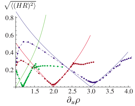
FIG. 10. (Color online) Comparison of numerical mean curvature variance \sqrt{\langle(HR)^2\rangle} (dashed lines are meant to guide the eyes between the data points) to analytical predictions (solid) for \rho_1 , t/w=0.025 as a function of \partial_u\rho=\cosh(u_0/R) for two-, three-, and four-wrinkle strips (green, red, and blue, respectively) — note the observed resonance minima at roughly \partial_u\rho=1.193 , \partial_u\rho=1.997 and \partial_u\rho=3.073 , compared to analytical predictions of \partial_u\rho=1, 2 , and 3 , for two-, three- and four-wrinkle strips, respectively.
