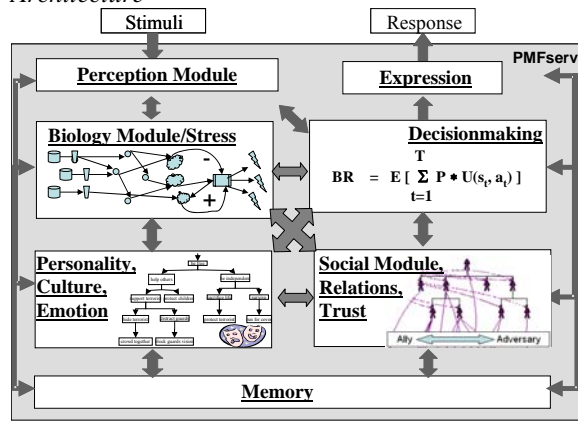
Figure 3 – PMFserv, an example Cognitive Architecture
