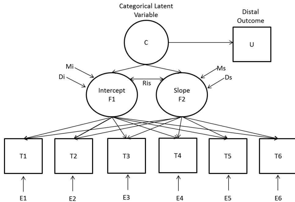
Figure 2. Representation of the latent variable growth mixture model, with latent subpopulations predicting a distal outcome.
