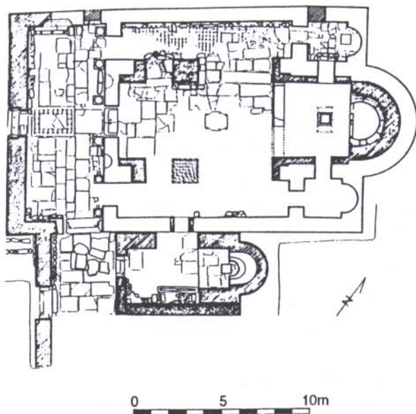
Figure 10.7 Selçukler, church, plan (Fıratlı).
