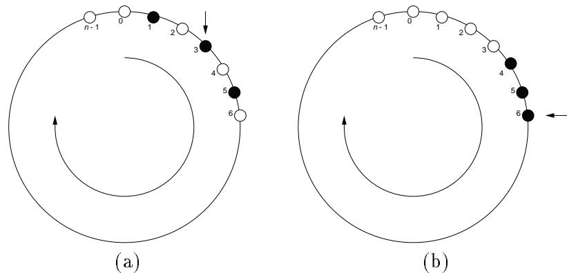
Figure 1: Examples of client configurations. Black circles represent cached pages and the outer arrow the algorithm position.
