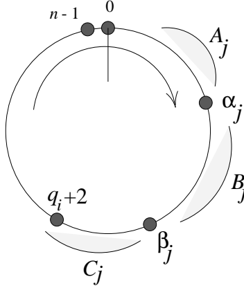
Figure 2: Lower bound for randomized algorithms without prefetching
