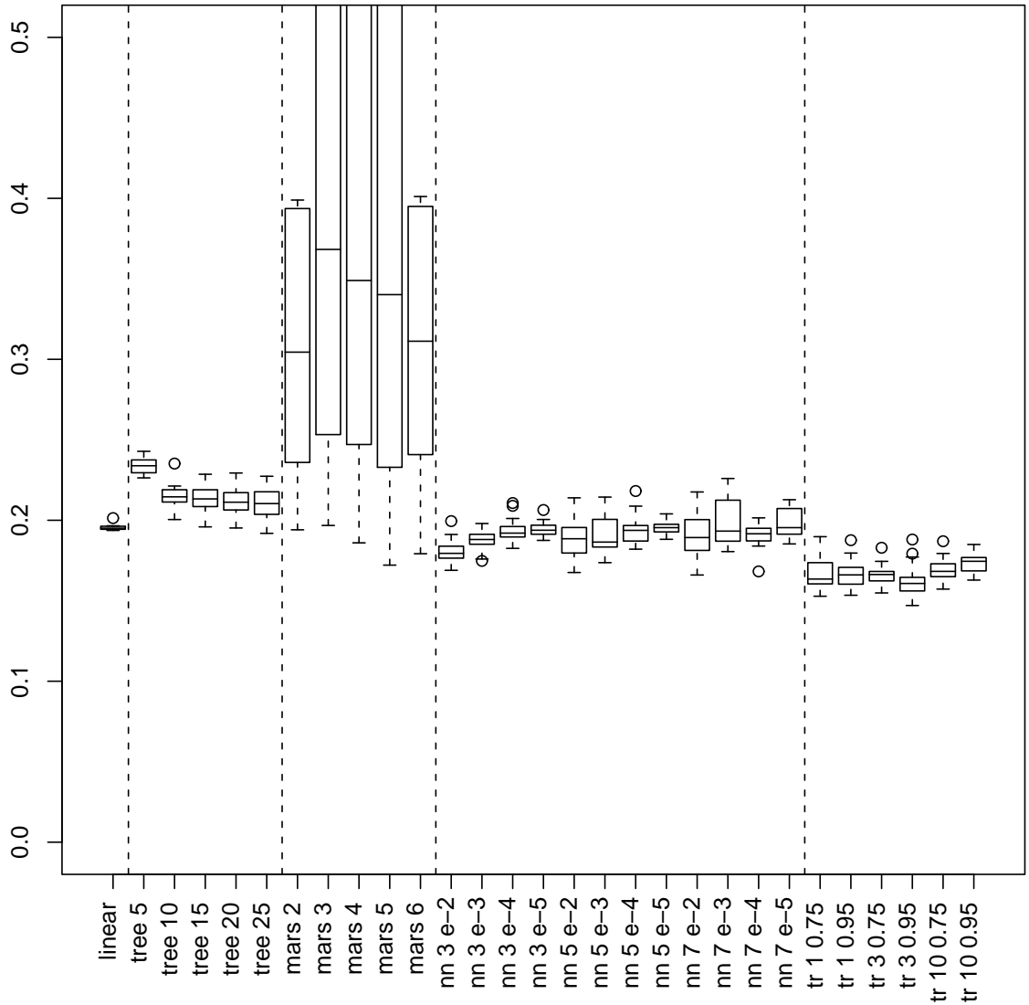
Figure 9: RMSE for test data, Boston Housing example
