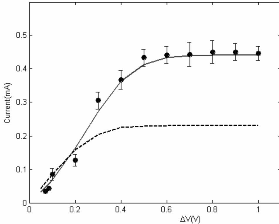
Fig.5: The steady state current as a function of the difference in the electrodes' potentials when the average electrolyte's concentration is 0.1M FeCl 3 and 0.1M FeCl 2 . The solid circles with error bars correspond to experimental data. The solid and dashed lines correspond, respectively, to theoretical predictions accounting for and neglecting natural convection effects.
