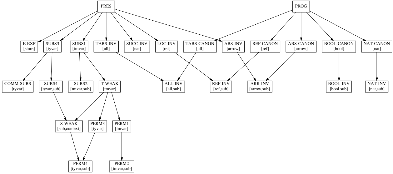
Figure 9: Preservation and Progress theorems and their lemmas
