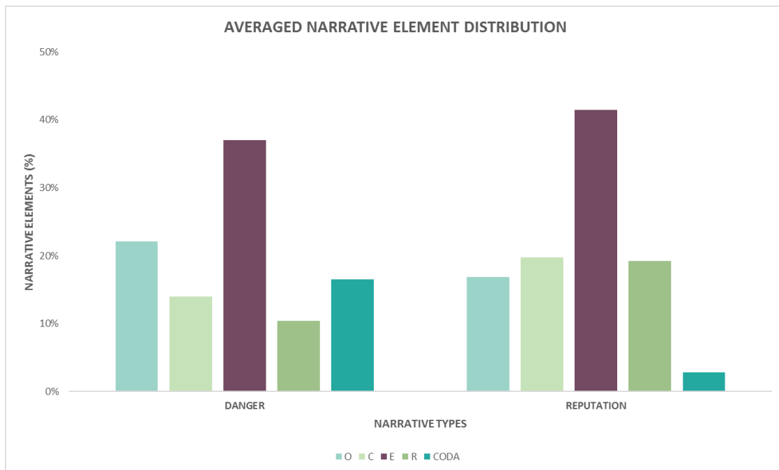
Figure 4: Averaged Distributions
