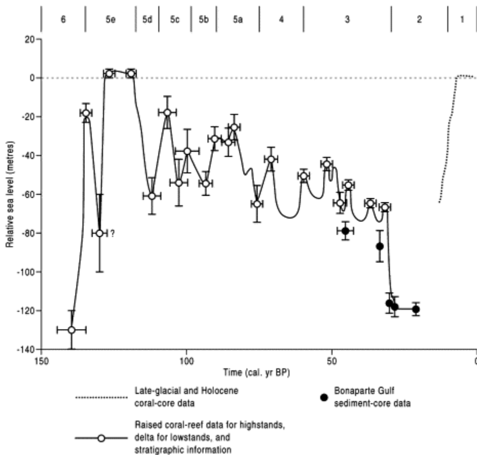
Fig. 1. The relative sea-level curve for the last glacial cycle for Huon Peninsula (Lambeck and Chappell, 2001) supplemented with observations from Bonaparte Gulf, Australia ( Yokoyama et al., 2000). Error bars define the upper and lower limits (modified from Lambeck et al., 2002).
