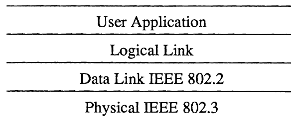
Figure A.2. Layers in RoboNet
