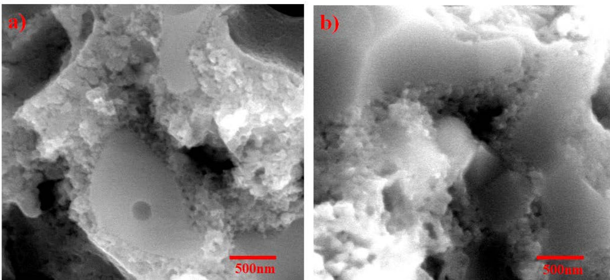
Figure S1: SEM images of bare LSF particles (a) and 100 cycles La modified LSF particles (b) on YSZ scaffold.
