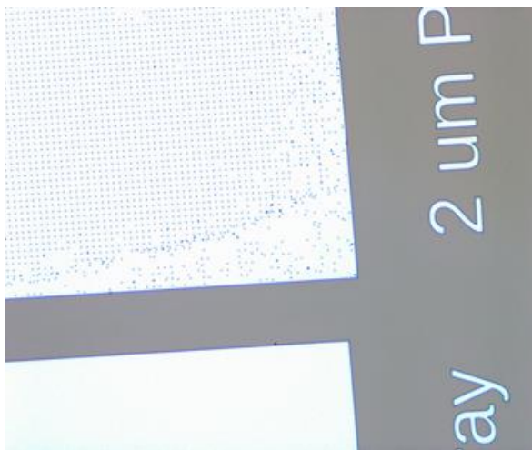
Figure 7: Poor adhesion of 2 µm pillar array
