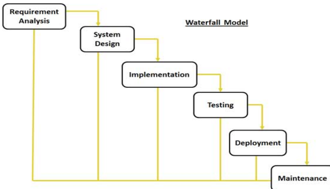
Figure 5. Common Waterfall System Development Life Cycle (SDLC) Model
