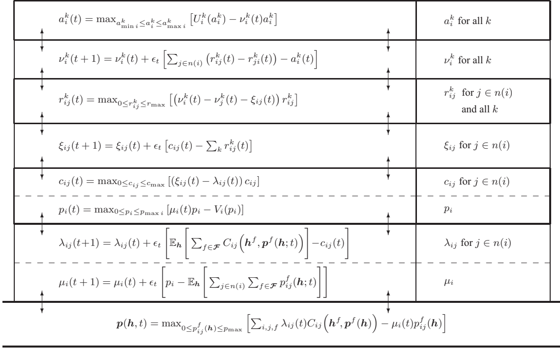
Fig. 2. The subgradient descent iteration (22)-(30) can be interpreted in terms of layers and layer interfaces. Layers keep variables of interest to the network, e.g., link transmission rates r_{ij}^k at the network layer, that they update according to primal iterations (22)-(26). Layer interfaces maintain (auxiliary) dual variables updated as per the dual iterations (27)-(30). Communication of variables across layers and interfaces is restricted to adjacent entities; i.e., layers receive variables from, and transmit to, adjacent interfaces. Interfaces exchange variables with adjacent layers. Note that in general the physical layer optimization problem cannot be separated in per-terminal problems.
