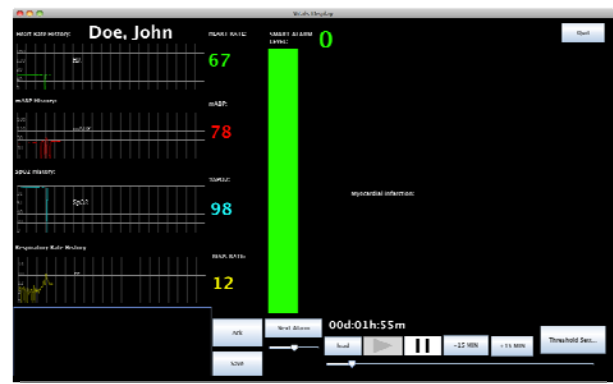
Figure 4: Java Implementation of the Smart Alarms App
