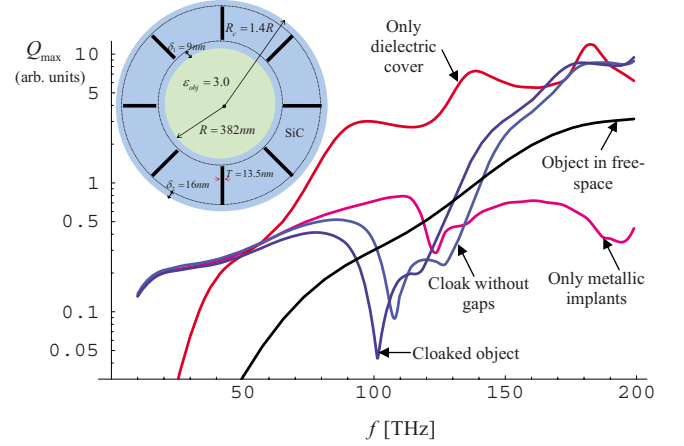
FIG. 4. (Color online) Peak in the scattering width Q (normalized to arbitrary units) as a function of frequency, for different scenarios of interest. The inset represents a combined object-cloak system (the different parts of the cloak are not drawn to scale).
