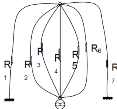
Figure 2: Simulated mine tunnel network
