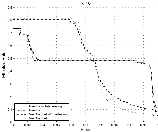
Figure 3: Channel Scenario 2: Two “average” channels. LT\epsilon R_1=11.39\% , EBL_1=11.1 , LT\epsilon R_2=9.83\% , EBL_2=5.0 .
