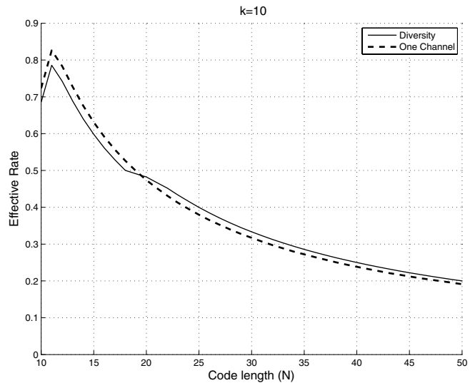
Figure 4: Channel Scenario 3: One “average” channel and one “good” channel. LT\epsilon R_1=11.27\% , EBL_1=10.9 , LT\epsilon R_2=4.17\% , EBL_2=1.1 .
