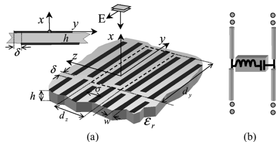
Fig. 1. Geometry of a gangbuster-FSS printed on a dielectric slab. h = 0.508 mm, w = 0.25 mm, d_y = 10 mm, \delta = 0.2 mm, d_z = 0.5 mm, relative permittivity of the slab \epsilon_r = 4.5 . Dipoles are printed on both sides of the dielectric slab. Inset at the left: transverse cross section showing the offset of dipoles placed at the same z -level. (b) Equivalent x -transmission line circuit network.
