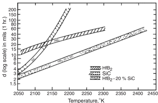
Fig. 1. One-hour oxidation resistance of monolithic \text{HfB}_2 , monolithic \text{SiC} , and \text{HfB}_2+\text{SiC} composite (taken from Clougherty, Pober, and Kaufman). 7
