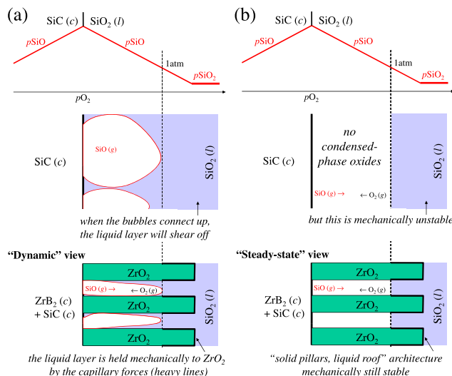
Fig. 2. The “dynamic view” (a) and “steady-state view” (b) of why \text{ZrB}_2+\text{SiC} has better oxidation resistance than monolithic \text{SiC} above the \text{SiO} boiling transition temperature.
