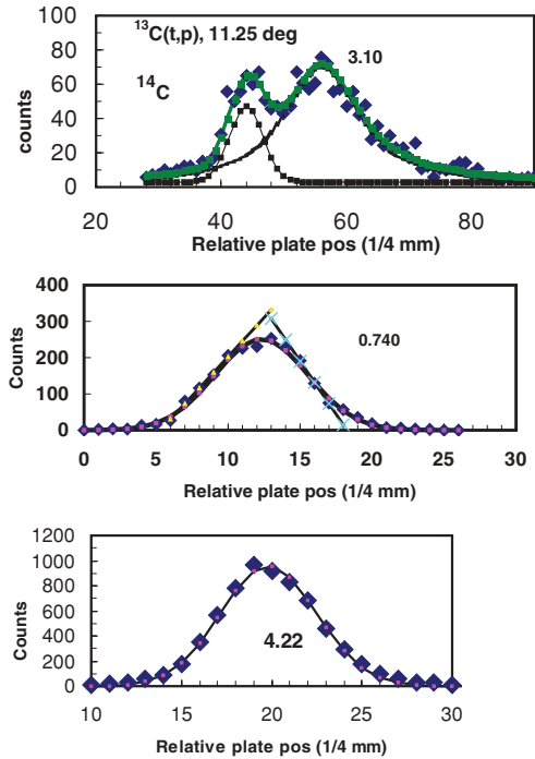
FIG. 1. (Color online) Peaks for three states of ^{15}\text{C} : the middle shows E_x = 0.740 , which is bound, the top is 3.105 , which has natural width, and the bottom has 4.22 , which is unbound but narrow. Curves are explained in the text.
