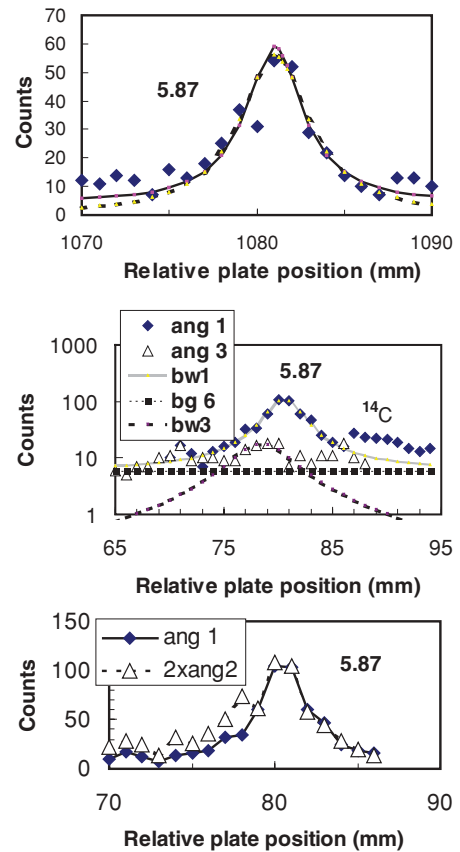
FIG. 3. (Color online) Data for 5.87\text{-MeV} region of ^{15}\text{C} at three forward angles. Top is for angle 2, bottom compares angles 1 and 2, and middle has angles 1 and 3. See the text.
