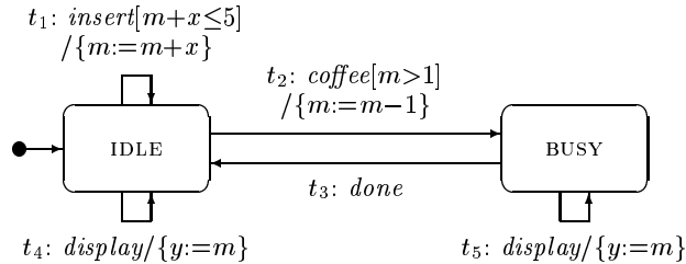
Fig. 1. An example of EFSMs
