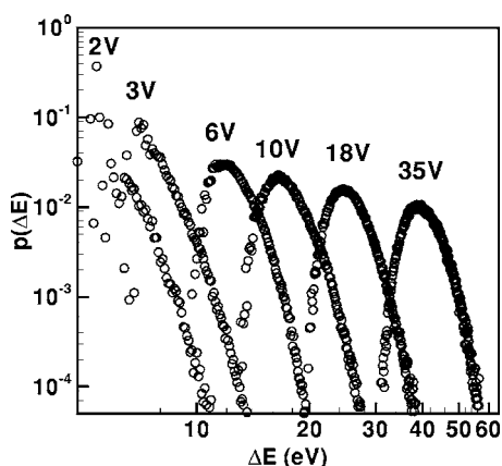
FIG. 7. Probability distribution function for vacancy clusters at 1600 K obtained directly from MD.
