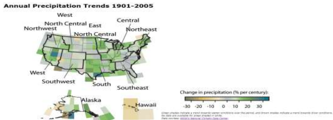
Figure 2: Annual Precipitation Trend in the US from 1901-2005. [2]
