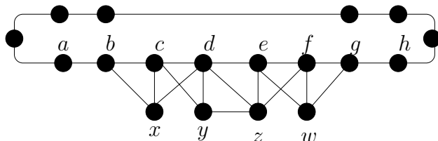
Figure 2: This graph is hunter-win against reactive rabbits but not against general rabbits.
