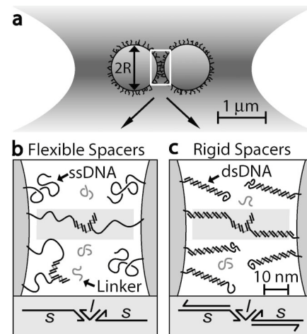
FIG. 1. (a) represents two microspheres trapped in the focal plane of a line optical tweezer. (b) shows microsphere surfaces chemically grafted with oligonucleotides, s , (sequence: ACTTA ACTACAGCATTATCAGTCTCCGAGGCCATTG-ATTCACACACGTCTAACTTGAATCTCT). Linker oligonucleotides, l , (sequence: AGAGATTCAAGTTCAGAGATTTCAAGTT) can bridge between microspheres (shaded boxes) after hybridizing with the terminal 14 bases of s (bold sequence). (c) same as (b) after hybridization of a third oligonucleotide complementary to s (underlined sequence), forming a rigid rodlike spacer.
