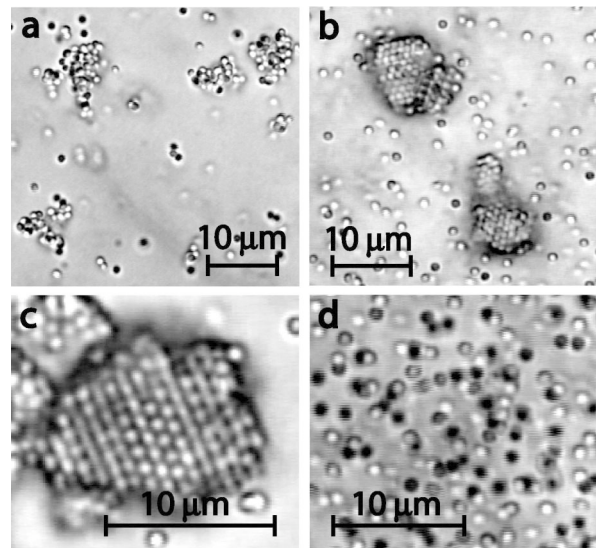
FIG. 3. Optical micrographs of colloidal microspheres assembled by DNA hybridization. (a) Colloidal spheres with \sim 14\,000 DNA/sphere on a CML surface formed only fractal-like aggregates after 96 h. (b) Similar spheres with \sim 3700 DNA/sphere on a PEG surface formed crystallites, shown after 96 h of growth. (c) A close-up of the front surface of one of the crystallites. (d) All crystallites and aggregates melted immediately upon heating by 2^\circ \text{C} , confirming they are held together by DNA bridges.
