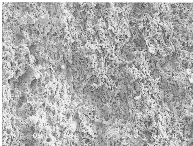
Fig. 3. SEM micrographs of 50:50 NiO/YSZ composite after acid leaching.
