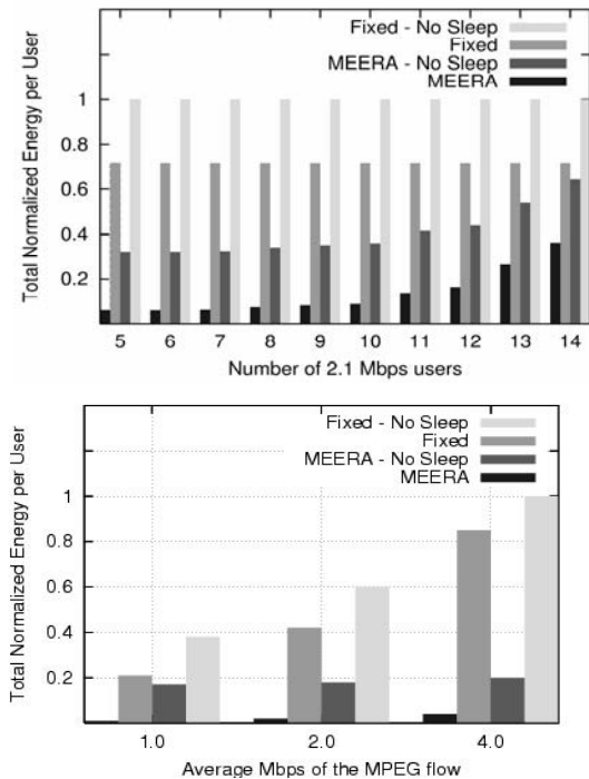
Figure 13 (a). Energy consumption per flow as a function of the aggregate system load for CBR traffic (b) Energy consumption per flow as a function of mean per-flow data rate for MPEG traffic
