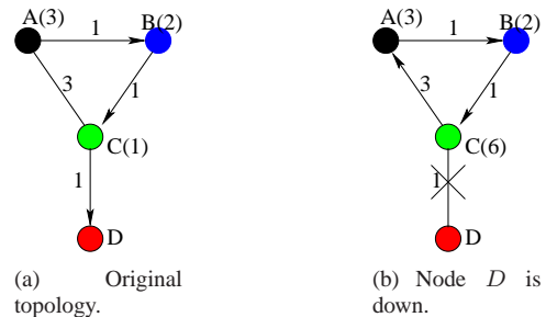
Fig. 1. A simple example of counting-to-infinity problem.
