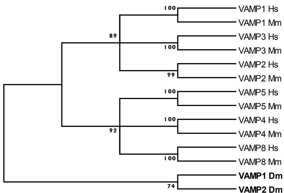
Maximum Parsimony
