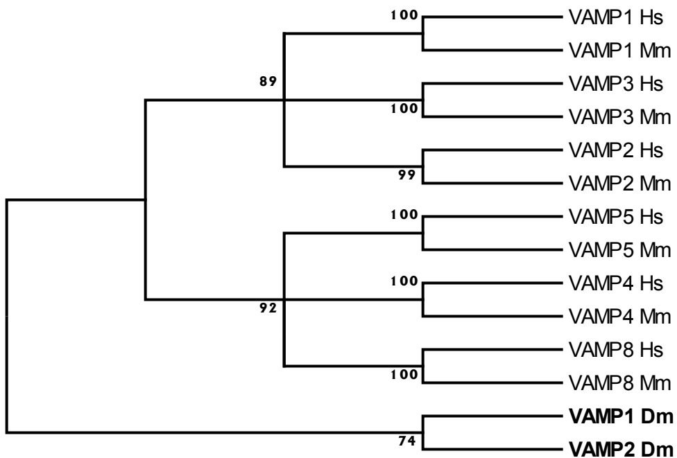
Neighbor-joining
