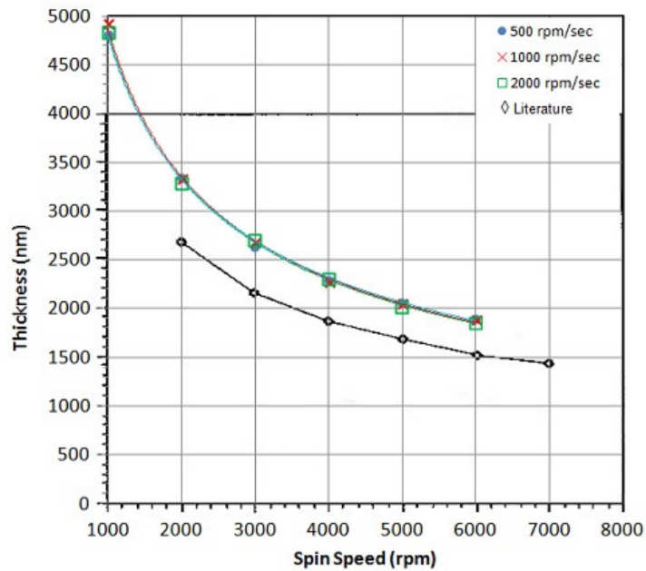
Spin Curve of S1818
