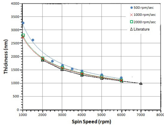
Spin Curve of S1813
