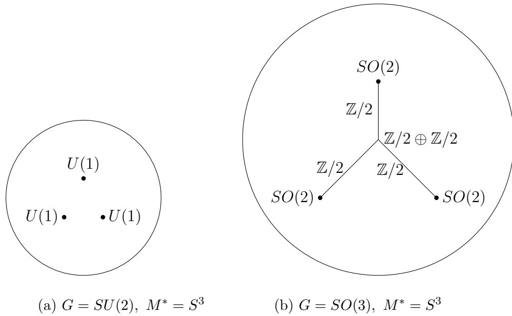
Figure 6.3: M = SU(3)/T^2
